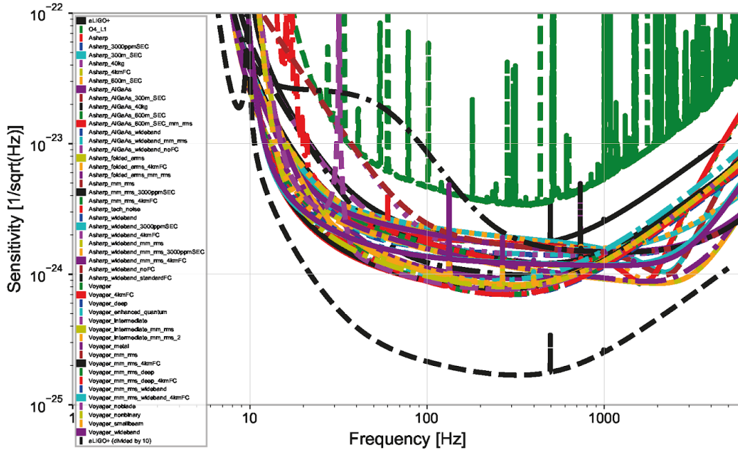
Figure A1.2: Amplitude Spectral Densities of the gravitational-wave-strain equivalent noise for various “advanced” observatory designs, showing the flexibility of possible designs .
