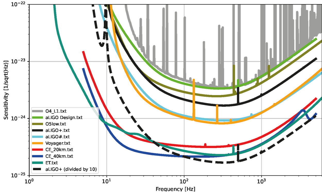
Figure 4.2: Amplitude Spectral Densities of the gravitational-wave-strain equivalent noise for various observatory designs. Note that the plot can only be indicative because the observatories and detectors in network configurations do not all respond to a certain type of gravitational wave in the same way. The responses differ depending on the incidence angle and polarization of the gravitational wave. Information on the sources for these curves can be found in Appendix A1.
