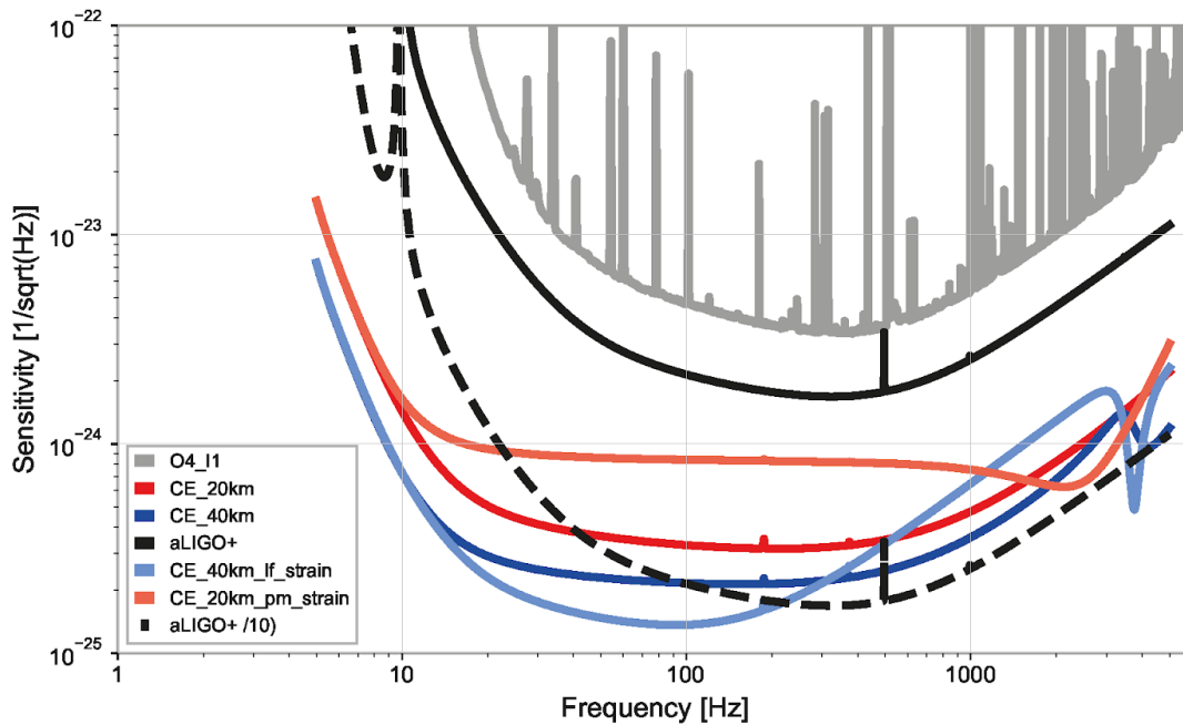
Figure A1.1: Amplitude Spectral Densities of the gravitational-wave-strain equivalent noise for various CE options (data from CE-T2000017 ) in comparison to O4, A+ and A+/10 sensitivities.
