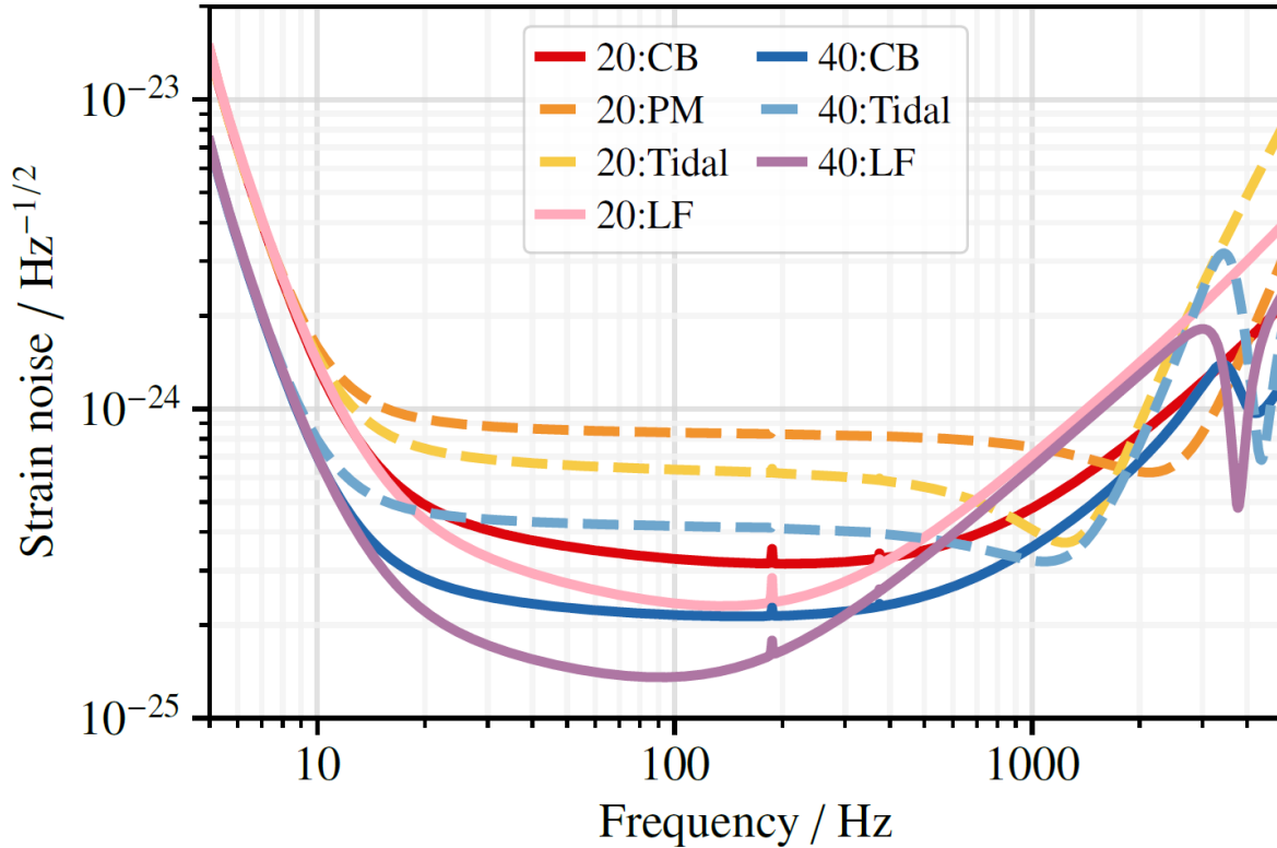
Figure 4.3: Amplitude Spectral Densities of the gravitational-wave-strain equivalent noise for various CE designs and tunings. xxii By changing the reflectivity and the tuning of the Signal Extraction Mirror, low- and mid-frequency performance can be traded against high-frequency performance. The compact binary (CB) configuration is the design sensitivity of the respective (40km or 20km) observatory. Each detector can be tuned to observe with a high-frequency optimized sensitivity post-merger optimized (PM) or binary neutron-star tidal (Tidal) and a low-frequency optimized sensitivity (LF).
